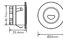
Cut-out: Ø45mm
