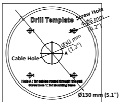
Figure 2-7 Drill Template
