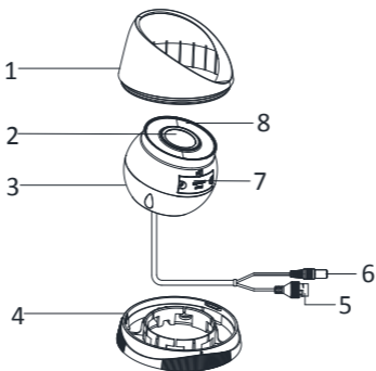
Figure 1-3 Type III Turret Camera Overview
